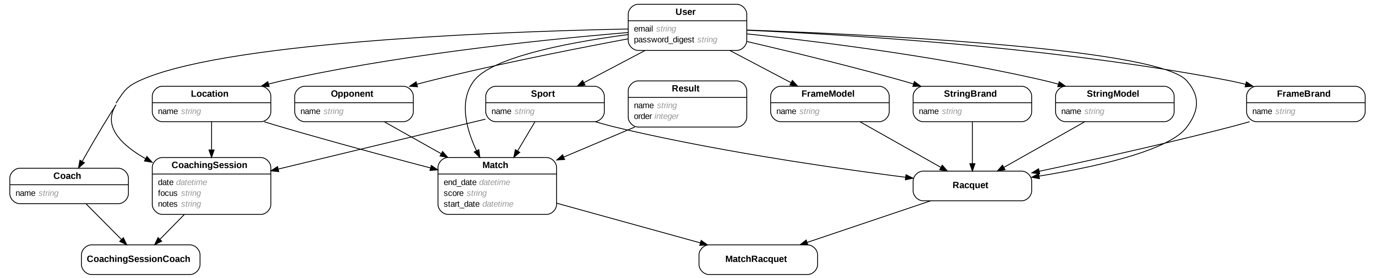
Racqueteer entity relationship diagram
